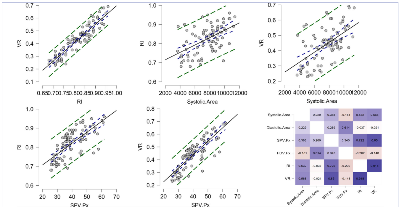
Figure 3. Regression lines between RI, VR, and systolic parameters and Pearson's r heatmap. RI: resistance index; VR: vascular resistance; SPV,px: mean of color pixel in systolic peak velocity.
