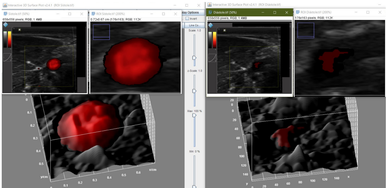
Figure 2. Quantification of vascular resistance by pixel color intensity from Power Doppler video with Doppler signal processing and calculation of mean of mean color pixels.
